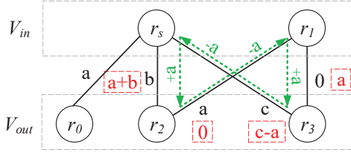
Fig. 4. The flow rule graph for S_2 in Fig. 3.
